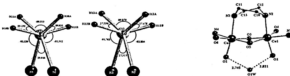
Figure 3. (a) Ethylene spacer within the piperazine ring is in gauche -conformation. (b) Hydrogen bonding interaction with suitably poised lattice water molecule in supramolecular structure further stabilizes the dimeric structure.
