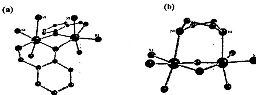
Figure 2. (a) The \text{Co}_2\text{O}_2 diamond core is presumably assembled as intermediate; (b) The core of complex 1 showing the fate of the piperazine backbone in twist-boat conformation
